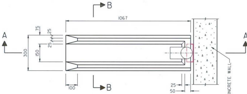
PLAN SCALE 1:5
