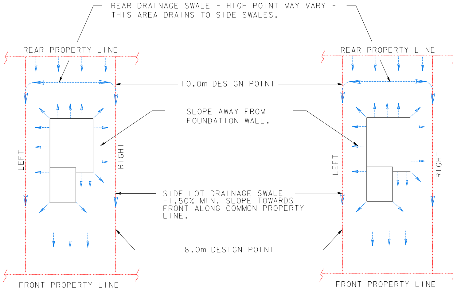
SINGLE FAMILY RESIDENTIAL LOT TYPE B REAR TO FRONT SURFACE DRAINAGE 3-6% OVERALL SLOPE
